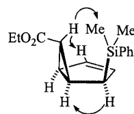
Figure 1. NOE effects in 7b (minor)
