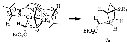
Figure 3. Transition state model for the asymmetric cyclopropanation of 6
