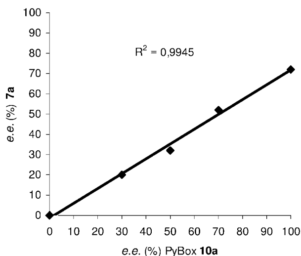
Figure 2. Variation of the ee of 7a as a function of the ee of ligand 10a
